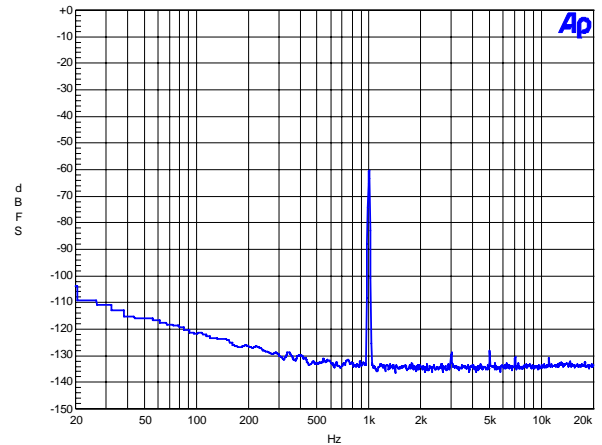
Figure 28. FFT (192 kHz, -60 dB)
